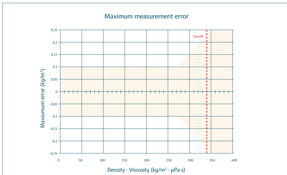
Graphic: Maximum measurement error
