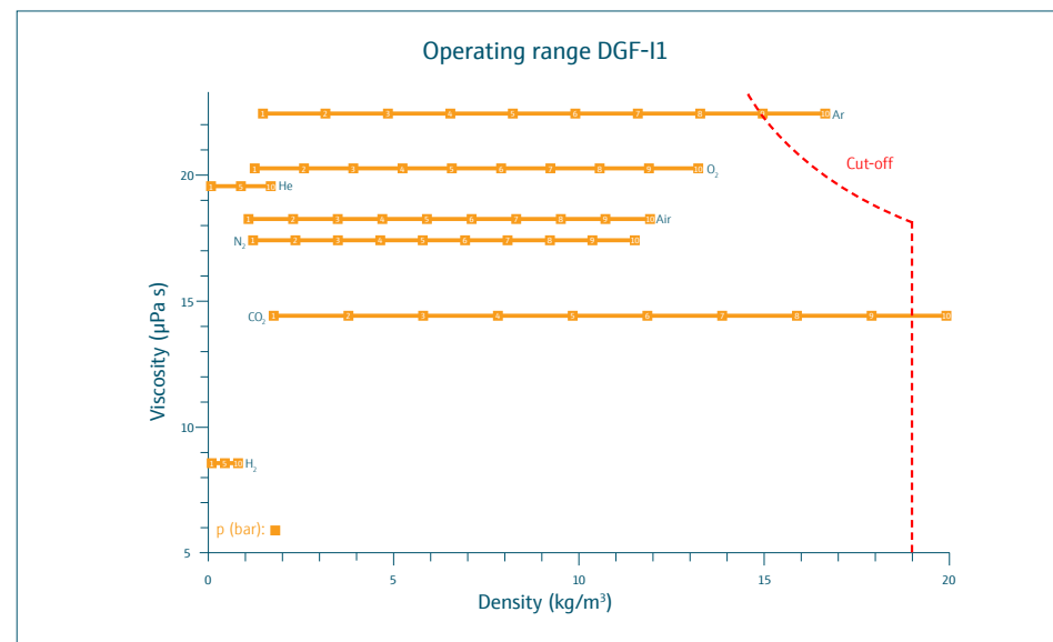
Graphic: Operating range DGF-I1
